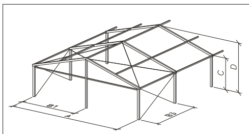
Truss-distance 5 m
